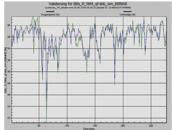
After implementing an optimization strategy, actual conditions closely correlate with the optimal set-points for wastewater treatment.
