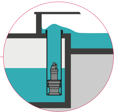
With a discharge pipe and free outlet.
