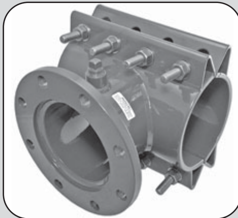
632 Tapping Sleeve
