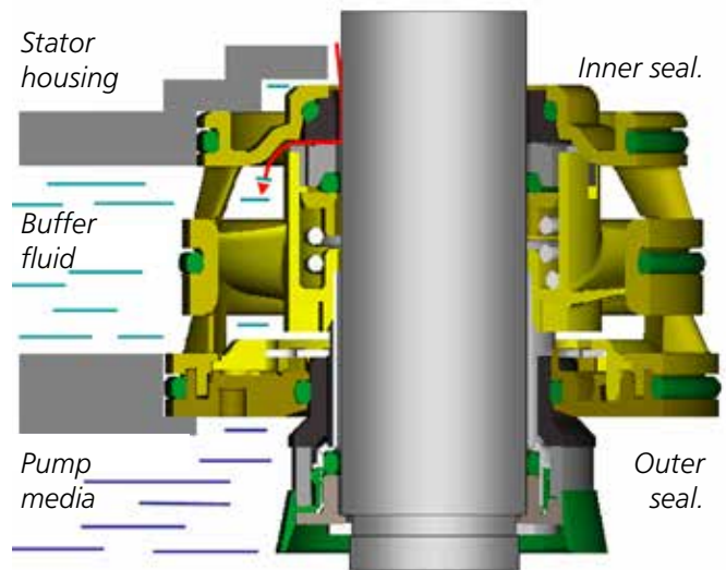
Active sealing applied in a Plug-In seal. Any buffer fluid that may leak into the stator housing is immediately pumped back to the buffer fluid chamber.
