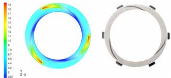
Pressure distribution in grooved seal face.
