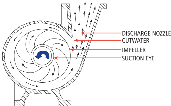
Impeller and Volute Interaction Figure 8
