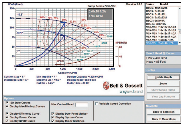
ESP Plus Pump Curve with Safety Factor System Curve Figure 55
