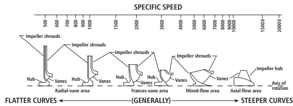
Specific Speed and Impeller Profile Figure 34
