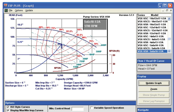
ESP Plus Pump Curve and System Curve Figure 54
