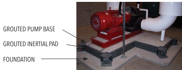
Typical Inertial Pad Installation Figure 32
