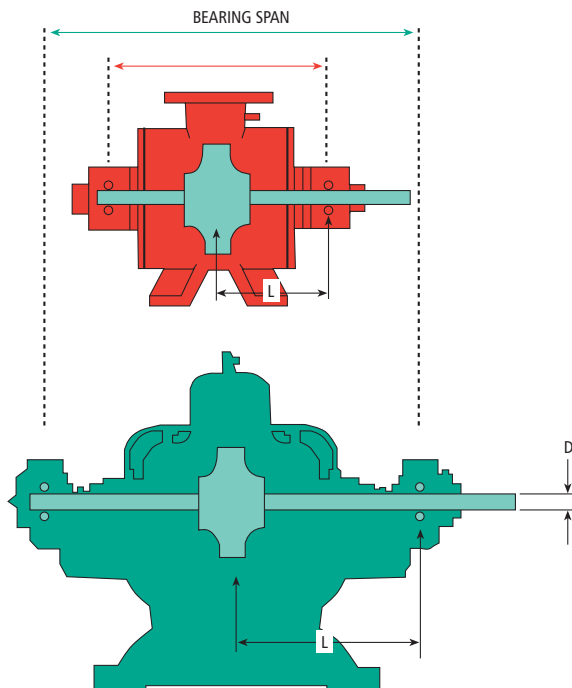
Bearing Span and Shaft Diameter Figure 48
