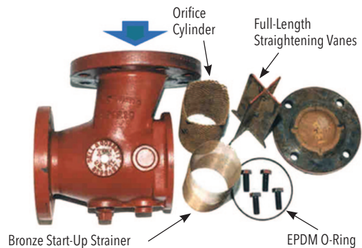
Suction Diffuser Internal Components Figure 28
