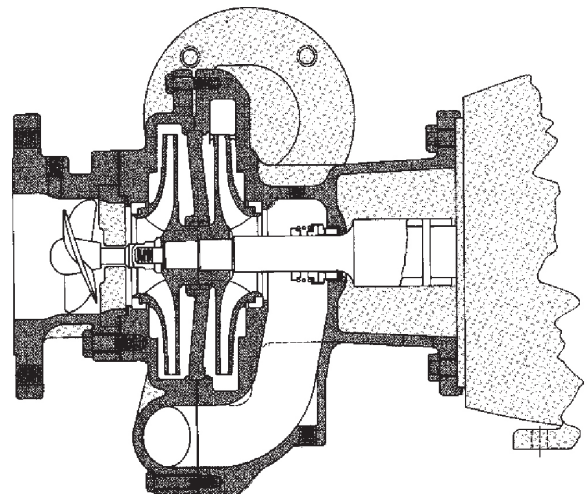
Domestic Series DB multistage pump Figure 20
