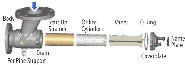
Exploded View, Suction Diffuser Internals Figure 29
