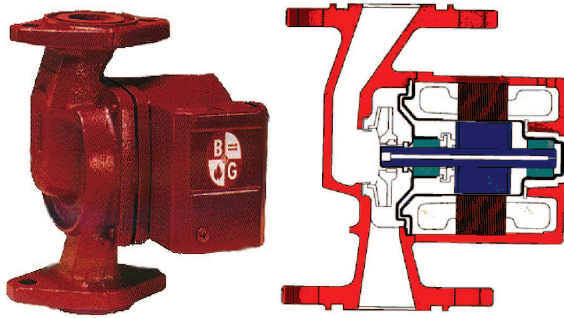
Series NRF Circulator Figure 18
