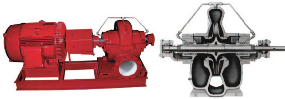
Horizontal Split Case, Double Suction Pump Figure 22
