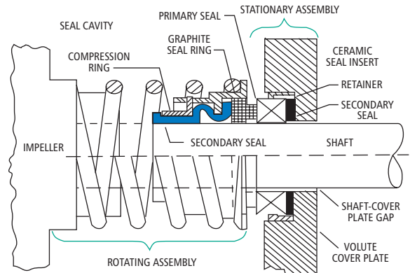
Typical Mechanical Pump Seal Figure 12
