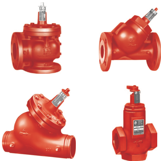
Triple Duty Valves in Various Connection Types and Sizes. The Valve at the Lower Right is Available up to 1½", the Rest are Available in Much Larger Sizes.
