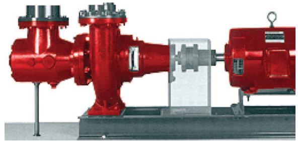
Suction Diffuser Installed on an End Suction Pump Figure 27
