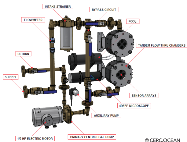
Fig. 1: Left: Design of the flow-through system onboard the Atlantic Condor. Right: Coupled SooGuard flow-through chambers. In the top chamber, open, the membrane of the modified CO 2 -Pro CV is seen with Aanderaa sensors mounted on the lid.
