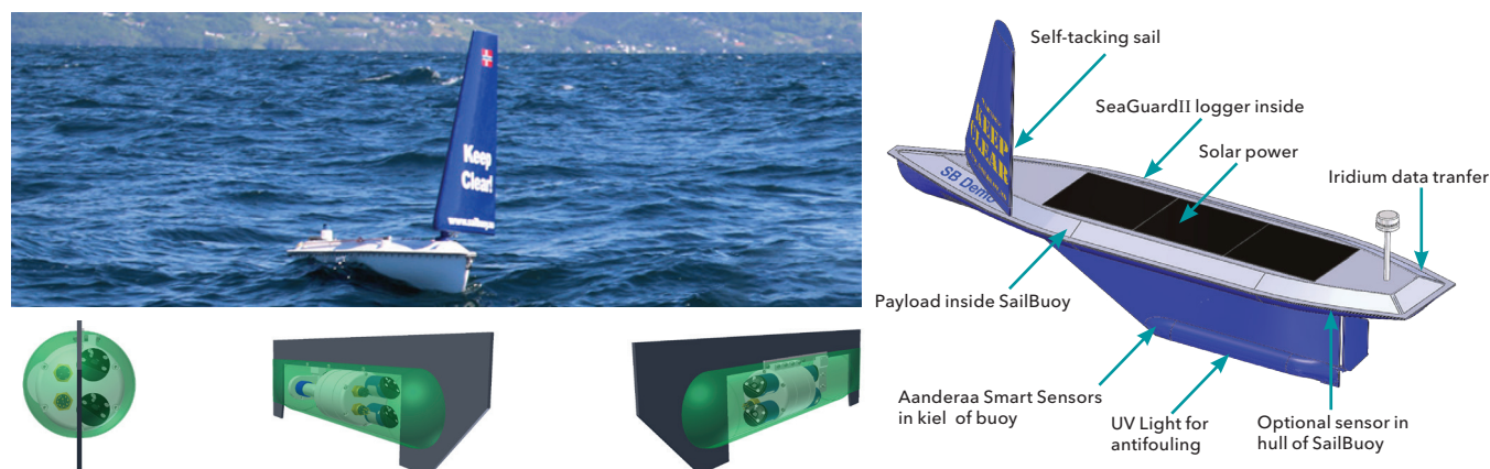
Fig. 3: SailBuoy with Aanderaa antifouling protected sensor package placed in the keel bulb
