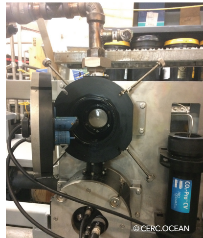
Fig. 1: Left: Design of the flow-through system onboard the Atlantic Condor. Right: Coupled SooGuard flow-through chambers. In the top chamber, open, the membrane of the modified CO 2 -Pro CV is seen with Aanderaa sensors mounted on the lid.
