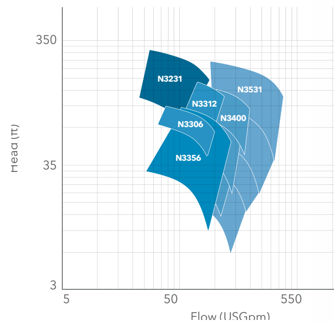
Performance, 60 Hz
